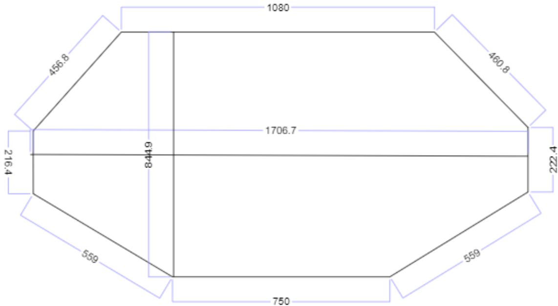
Zip Zap Dome Stage 1 – measurements are in Metres (m)
